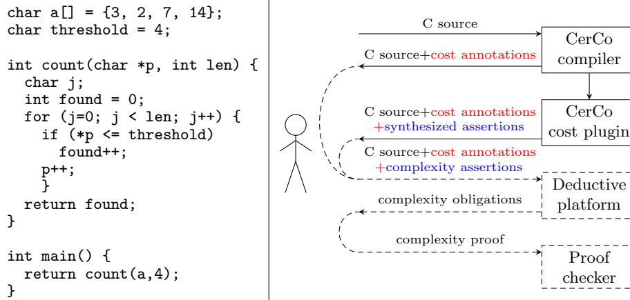
Fig. 1. On the left: code to count the array’s elements that are less than or equal to the threshold. On the right: CerCo’s interaction diagram. CerCo’s components are drawn solid.
